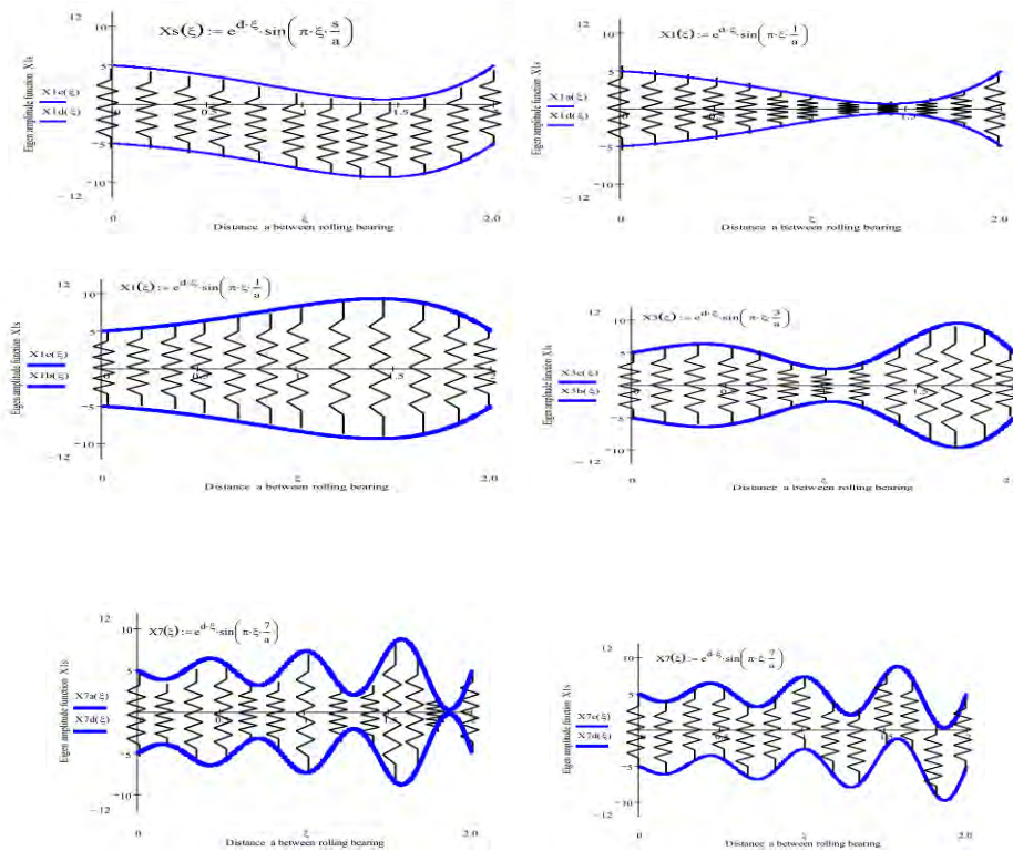
Figure. Sixth cases of the possible vibrations forms of the double belt system with elastic layer for different eigen amplitude functions
