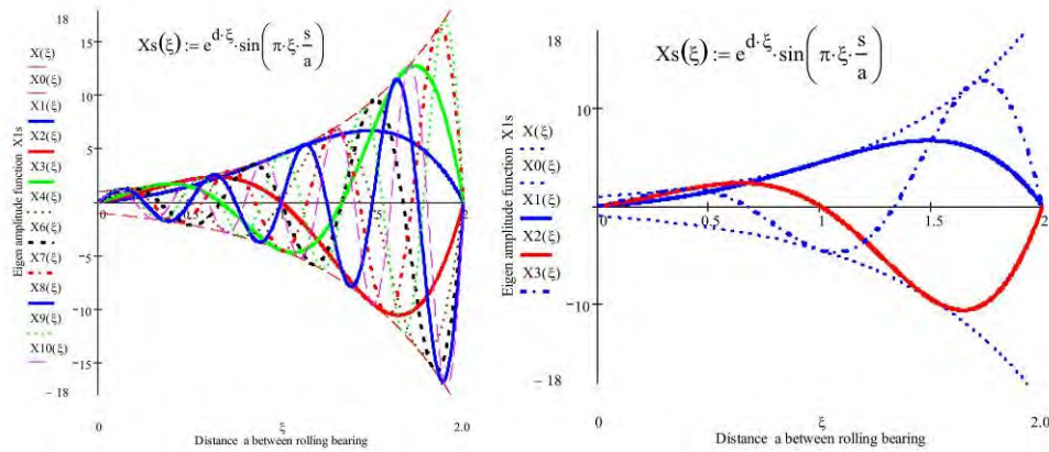
Figure. Eigen amplitude functions \mathbf{X}_{(i)s}(\xi) = e^{\tilde{d}\xi} \sin \frac{S}{\ell} for the solution in the \xi, \eta = \frac{V_0}{c_0^2 - v_0^2} x + t coordinates and for decoupled belts.
